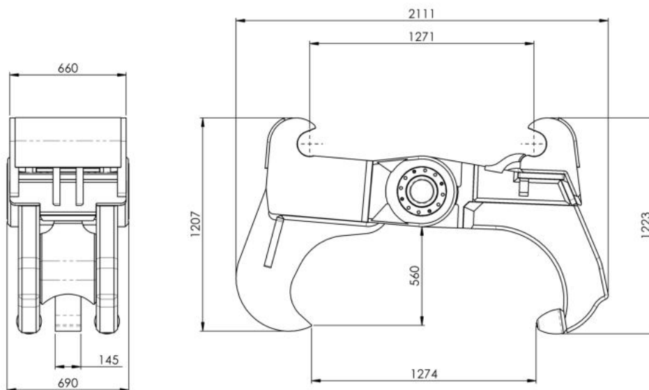
Tripod-Gebiss
